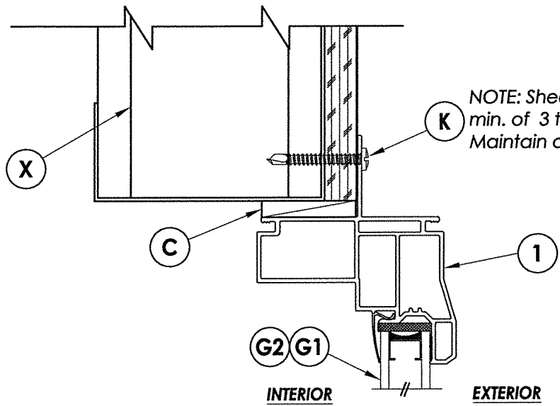
3 VERTICAL CROSS SECTION 3 Steel Stud Construction
