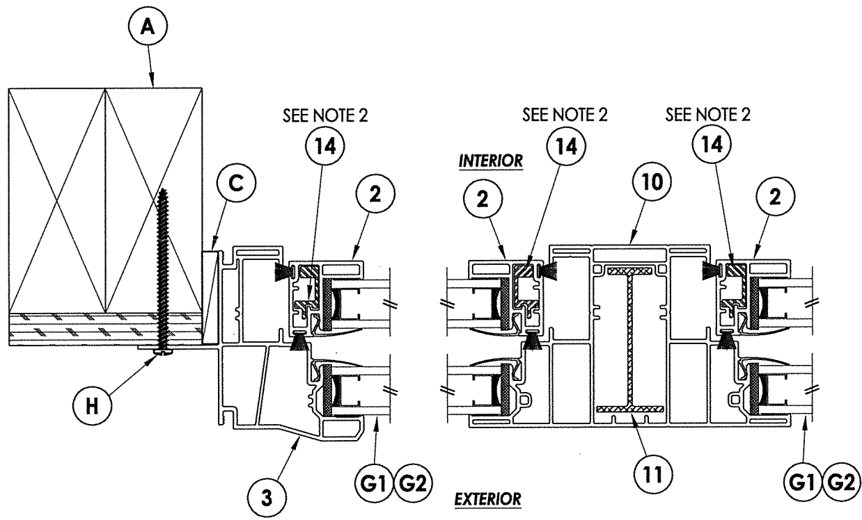
1 HORIZONTAL CROSS SECTION 3 Stud Construction
