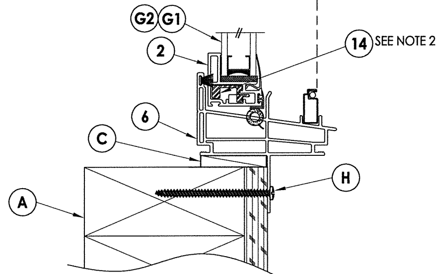
2 VERTICAL CROSS SECTION 3 Stud Construction
